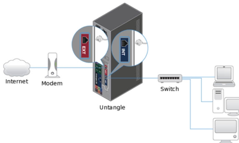
Router Mode Untangle serves as the router and the firewall
